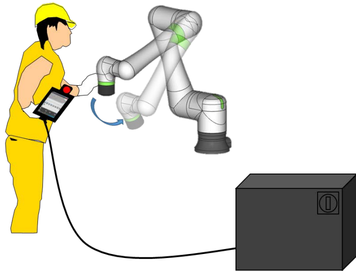
Fig. 4.5(a) Correct operation of manual guided teaching
