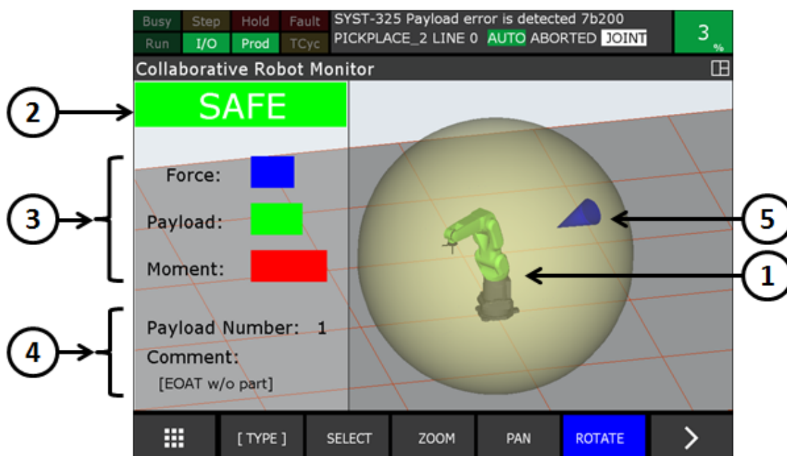
Fig. 8.4.1(a) Information on Collaborative Robot Monitor screen
