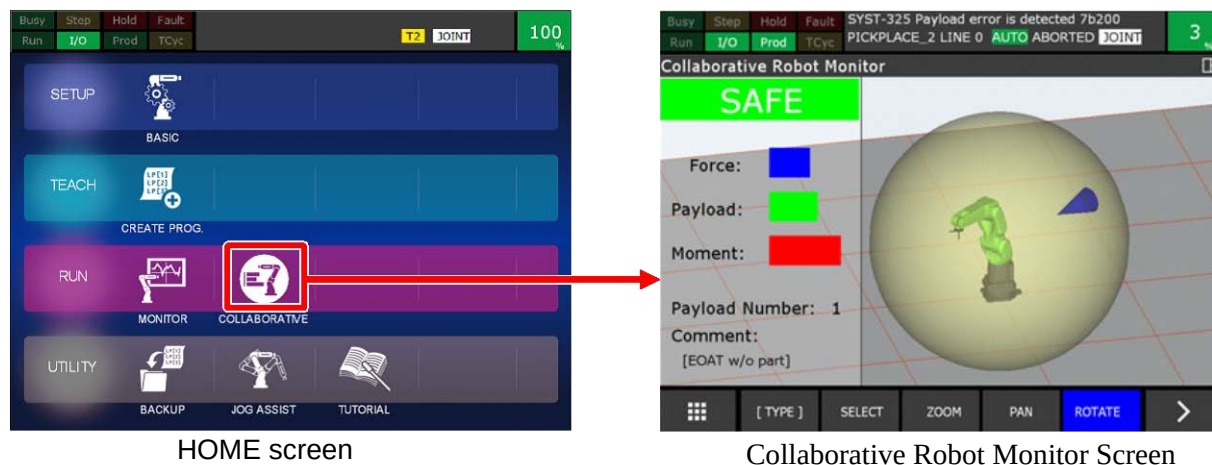
Fig. 8.4(a) Screen display flow (Collaborative Robot Monitor)
