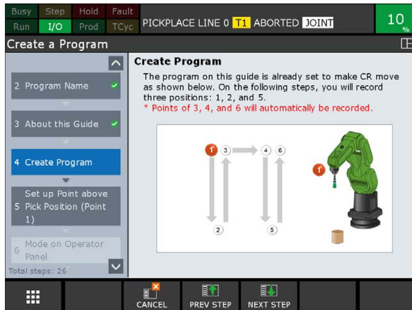
Fig. 8.3.2(a) Create a Pick & Place with light work screen
