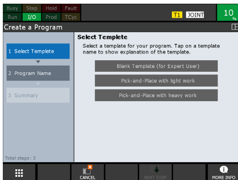
Fig.8.3.1(a) Create a Program Screen
